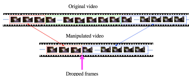
Figure 1: The illustration of frame dropping detection challenge. Assuming that there are three consecutive frame sequences (marked in red, green and blue, respectively) in an original video, the manipulated video is obtained after removing the green frame sequence. Our goal is to identify the location of the frame drop at the end of the red frame sequence and the beginning of the blue frame sequence.
